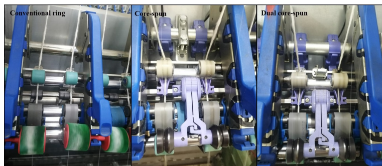
Figure 1: RS, CS and DCS yarn production frame
