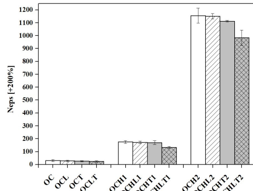
Figure 4: Thick places values of the yarns fabricated
