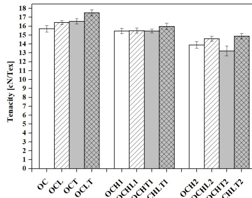
Figure 7: Yarn tenacity of the yarns fabricated
