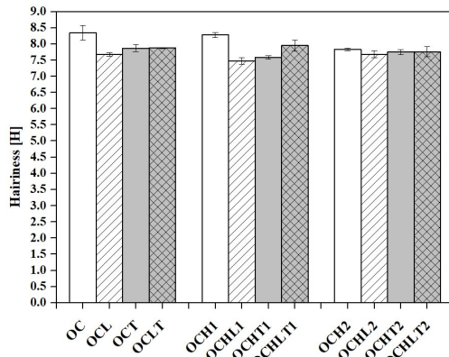
Figure 6: Yarn hairiness of the yarns fabricated
