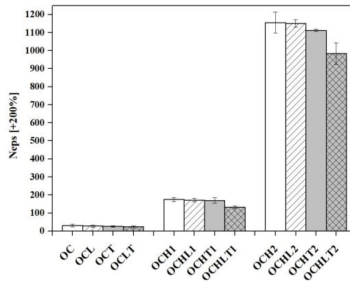
Figure 5: Nep values of the yarns fabricated
