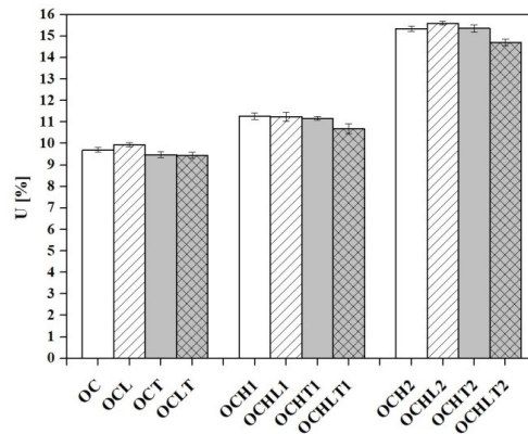
Figure 2: Yarn unevenness values of the yarns fabricated
