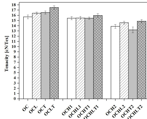
Figure 7: Yarn tenacity of the yarns fabricated
