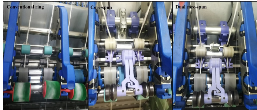
Figure 1: RS, CS and DCS yarn production frame
