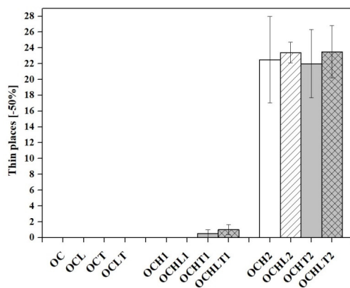
Figure 3: Thin places values of the yarns fabricated
