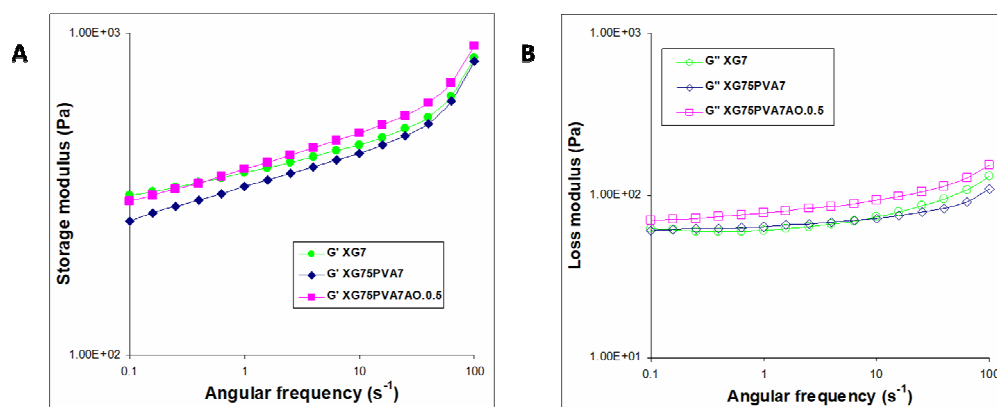
Figure 5: Variation of (a) storage modulus ( G' ) and (b) loss modulus ( G'' ) as a function of angular oscillation frequency at 25 °C for systems containing 75% XG after 7 freeze/thawing cycles
