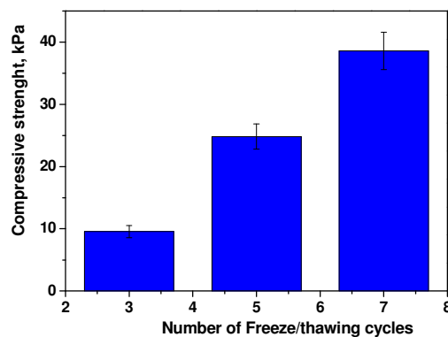
Figure 3: Compressive strength of RGP containing XG/PVA cryogels as a function of the number of freeze/thawing cycles
