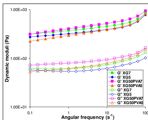
Figure 4: Influence of freeze/thawing cycles on the variation of storage modulus ( G' ) and loss modulus ( G'' ) as a function of angular oscillation frequency at 25 °C for XG and systems containing 50% XG
