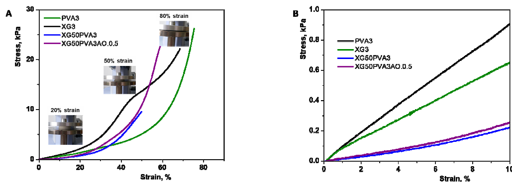
Figure 2: (A) Representative compression stress-strain curves for XG/PVA cryogels obtained in three freeze/thawing cycles under uniaxial compression (optical pictures from the insets correspond to XG50PVA3 sample); (B) Linear dependence of stress-strain curves from which the elastic moduli of all composites were calculated
