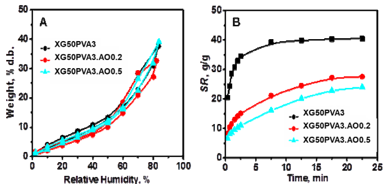
Figure 6: (A) Sorption and desorption isotherms of XG/PVA cryogels prepared using an XG:PVA ratio of 50:50, through 3 freeze/thawing cycles, without RGP (XG50PVA3) and with RGP content of 0.2 wt% (XG50PVA3.AO0.2), and, respectively, of 0.5 wt% (XG50PVA3.AO0.5); (B) Swelling ratio (SR, g/g) of XG/PVA cryogels as a function of time (min)
