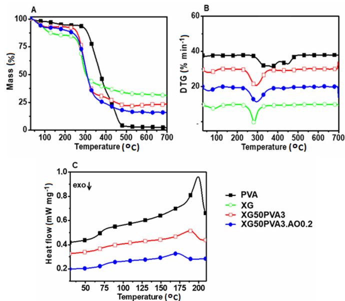
Figure 1: TGA (A), DTG (B) and DSC (C) curves of PVA, XG and of XG/PVA cryogels without (XG50PVA3) and with RGP (XG50PVA3.AO0.2)
