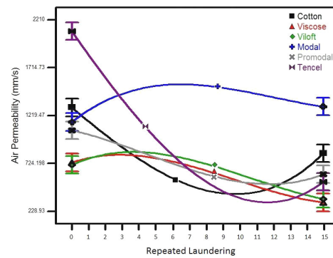
Figure 2: Regression curves for air permeability
