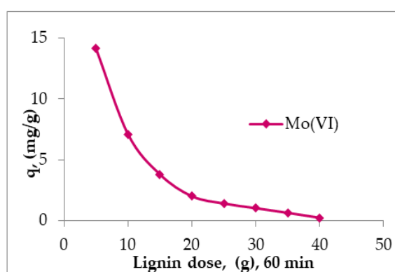
Figure 2: Influence of Sarkanda grass lignin dose on the adsorption of Mo(VI) at a concentration of 95.94 mg/L, at a contact time 60 min, pH 5.7
