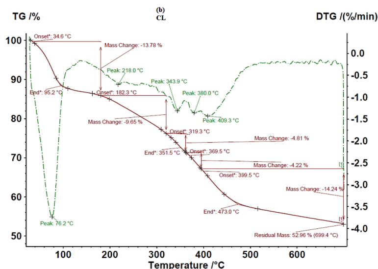
Figure 10: Thermogravimetric (red) and differential thermogravimetric (green) curves of Sarkanda grass lignin before (a) and after (b) Mo(VI) adsorption at a contact time of 60 min
