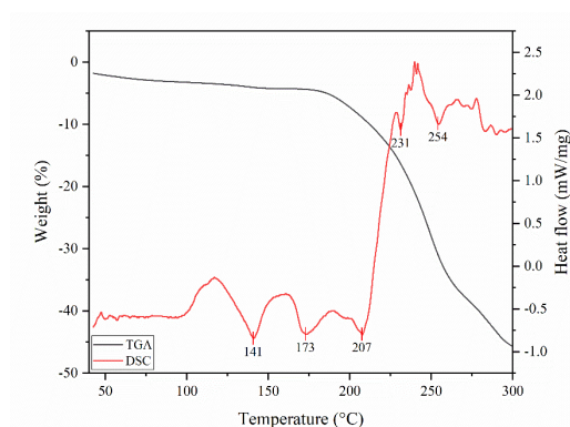
Figure 13: DSC-TGA thermogram of the optimal formulation
