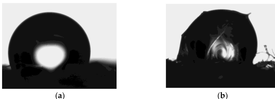
Figure 2: Visuals depicting contact angle measurements of (a) soap-washed wool fibers and (b) wool fibers exposed to peroxide treatment (adopted from ref. 49 with permission; Copyright 2022 MDPI Materials (Open Access Creative Commons CC-BY-NC 4.0 license)) 49
