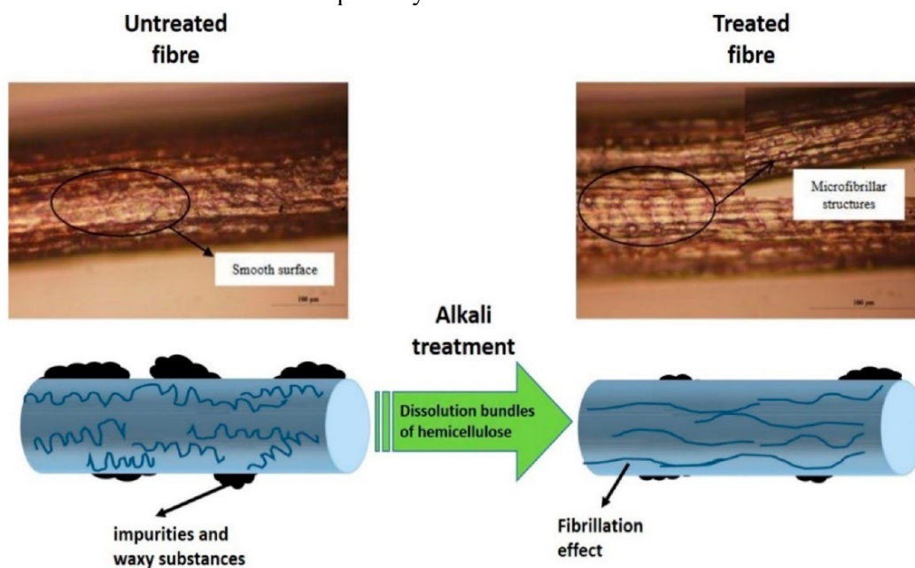
Figure 1: Schematic representation of natural fiber modification through alkaline treatment (adopted from ref. 47 with permission; Copyright 2022 MDPI Polymers (Open Access Creative Commons CC-BY-NC 4.0 license)) 47
