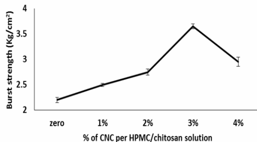
Figure 5: Effect of CNC addition on burst strength (Kg/cm 2 ) of composite films
