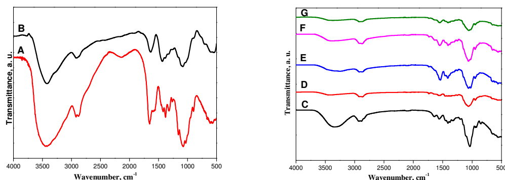
Figure 3: FT-IR spectra of chitosan (A), CNCs (B), chitosan/hydroxypropyl methylcellulose (C), after incorporation of CNCs (4%) and different menthol oil contents 0.35 (D), 0.4 (E), 0.6 (F) and 0.8 (G)
