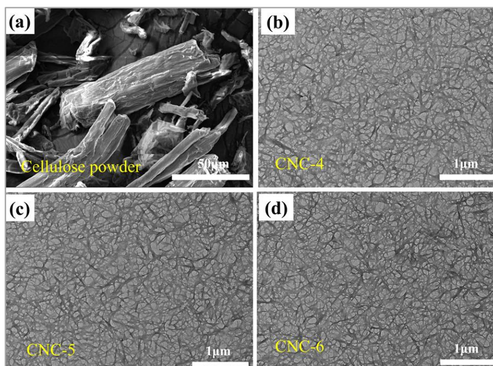
Figure 4: SEM image of cellulose powder (a) and TEM images of representative CNC samples (b-d)
