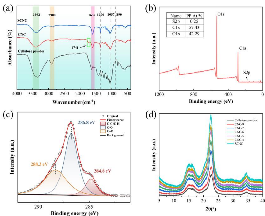
Figure 5: FTIR, XPS, and XRD analyses of cellulose powder, SCNC, and CNCs; (a) FTIR spectra, (b) XPS survey spectrum, (c) high-resolution C1s XPS spectrum, (d) XRD patterns
