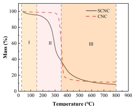
Figure 6: TG curves of CNC-4 and SCNC
