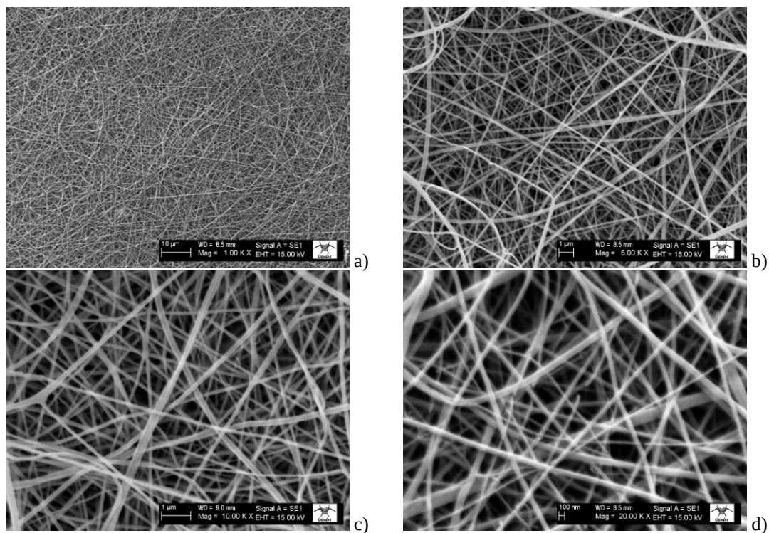
Figure 6: SEM images of P75 nanofiber surface samples at a) 1 kX, b) 5 kX, c) 10 kX and d) 20 kX
