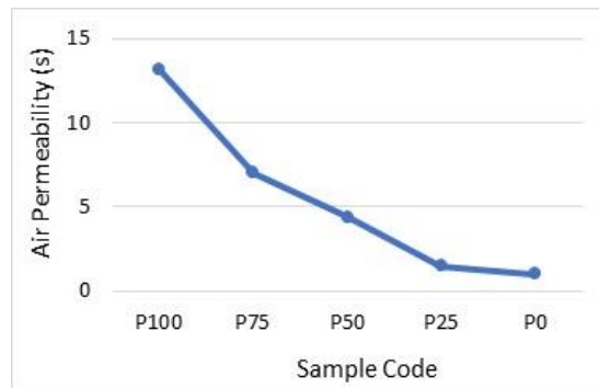
Figure 15: Variation of air permeability values of the produced nanofiber mats as a function of the PA6/CA mixing ratios
