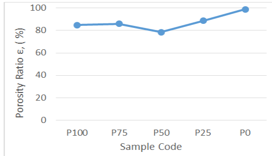
Figure 18: Variation of porosity ratio values of produced nanofiber mats as a function of PA6/CA mixing ratios
