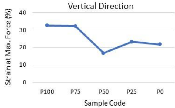
Figure 14: Variation of the strain at maximum force of nanofiber mats in cross-direction (V) relative to the collector
