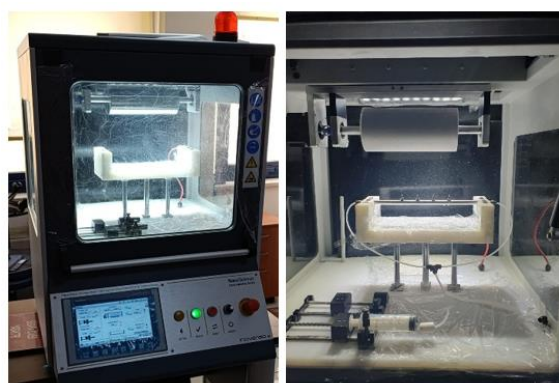
Figure 3: Inovenso NE300 model electrospinning device with a cylindrical collector
