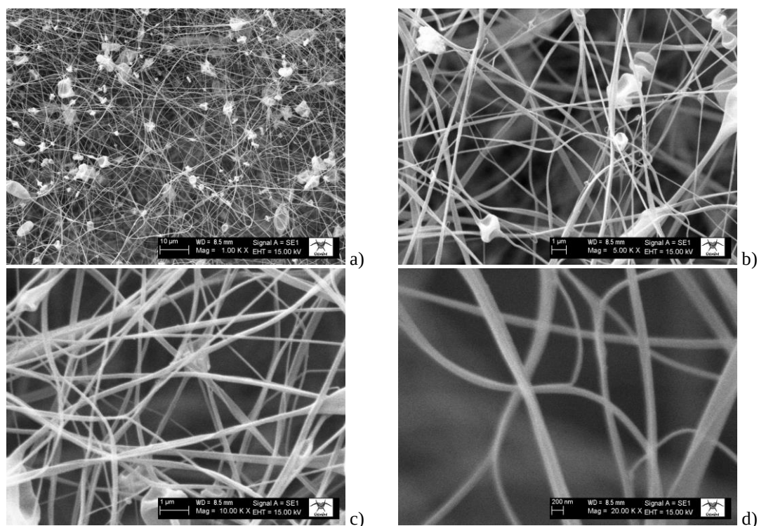
Figure 9: SEM images of P0 nanofiber surface samples at a) 1 kX, b) 5 kX, c) 10 kX and d) 20 kX
