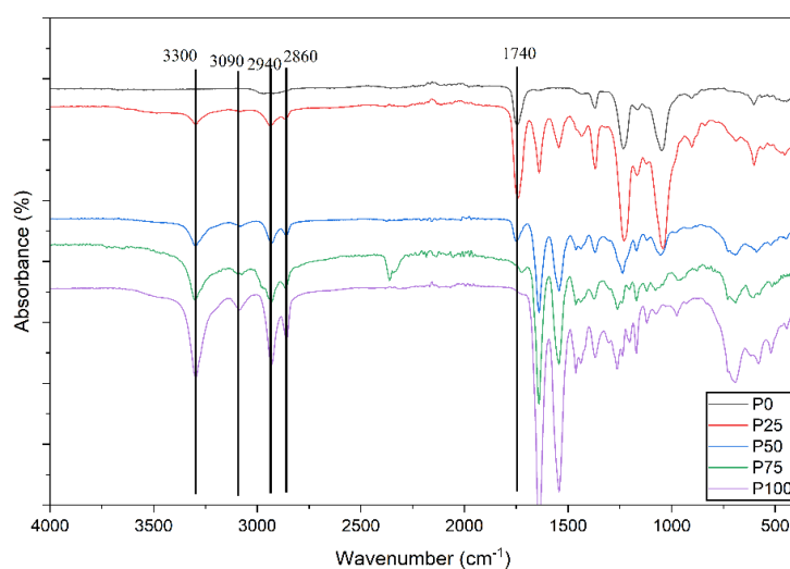
Figure 4: FTIR spectra obtained for formulations with different PA6/CA ratios
