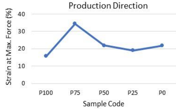
Figure 12: Variation of the strain at maximum force of nanofiber mats in the production direction (P)
