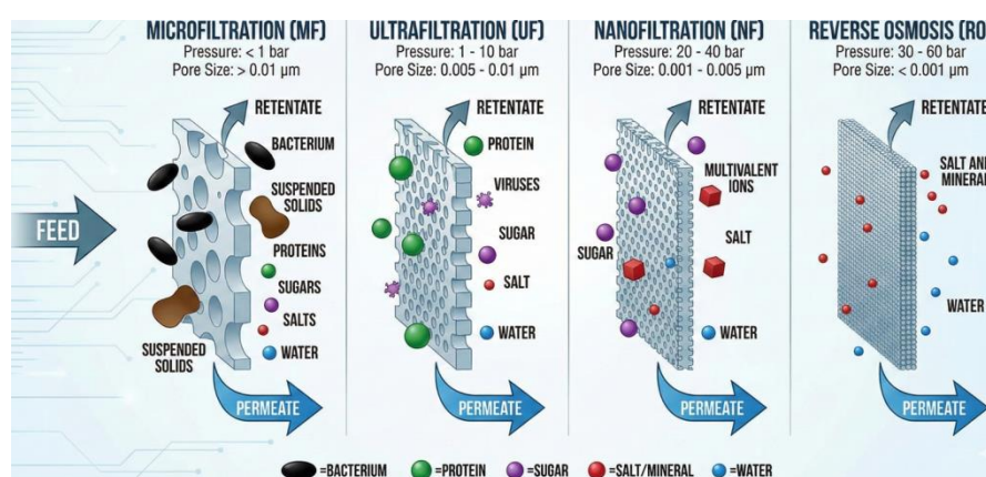
Figure 2: Classification of membranes based on their pore size and their retentate 5
