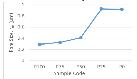
Figure 19: Variation of pore size values of produced nanofiber mats as a function of PA6/CA mixing ratios
