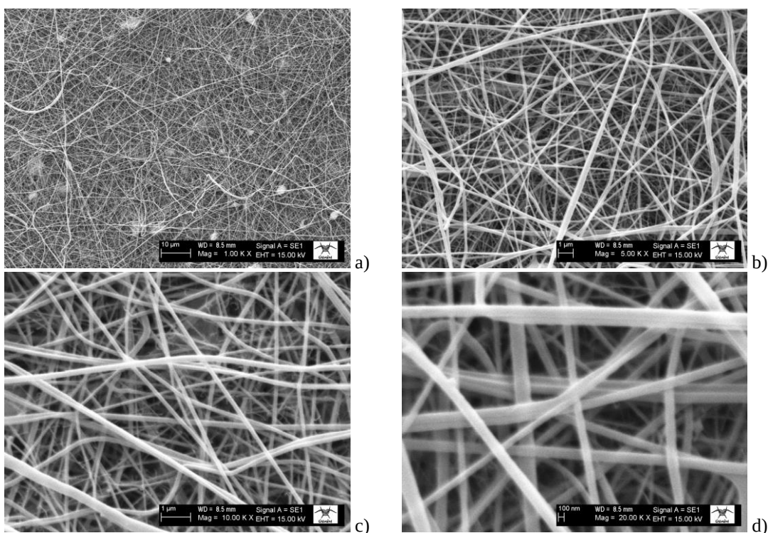
Figure 7: SEM images of P50 nanofiber surface samples at a) 1 kX, b) 5 kX, c) 10 kX and d) 20 kX
