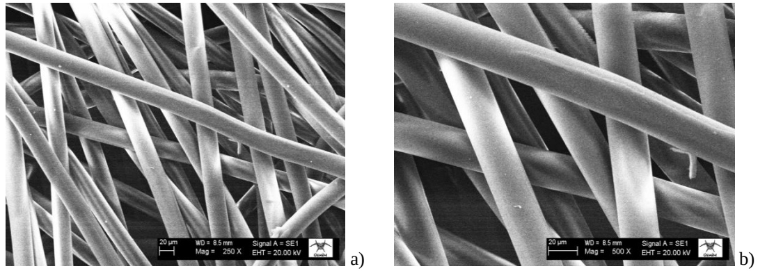
Figure 10: SEM images of spunbond fabric sample at a) 250 X, b) 500 X
