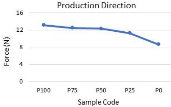
Figure 11: Variation of strength of nanofiber mats in the production direction (P)
