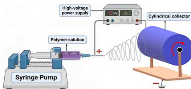
Figure 1: Basic components of an electrospinning system with cylindrical (rotating drum) collector
