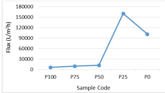
Figure 16: Variation of flux values of produced nanofiber mats as a function of PA6/CA mixing ratios
