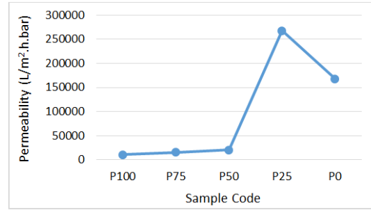
Figure 17: Variation of pure water permeability values of produced nanofiber mats as a function of PA6/CA mixing ratios
