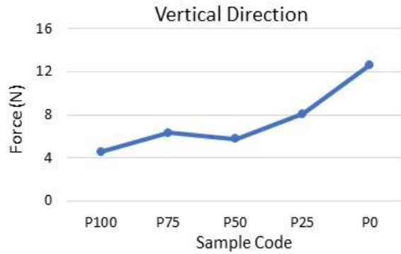
Figure 13: Variation of strength of nanofiber mats in cross-direction (V) relative to the collector
