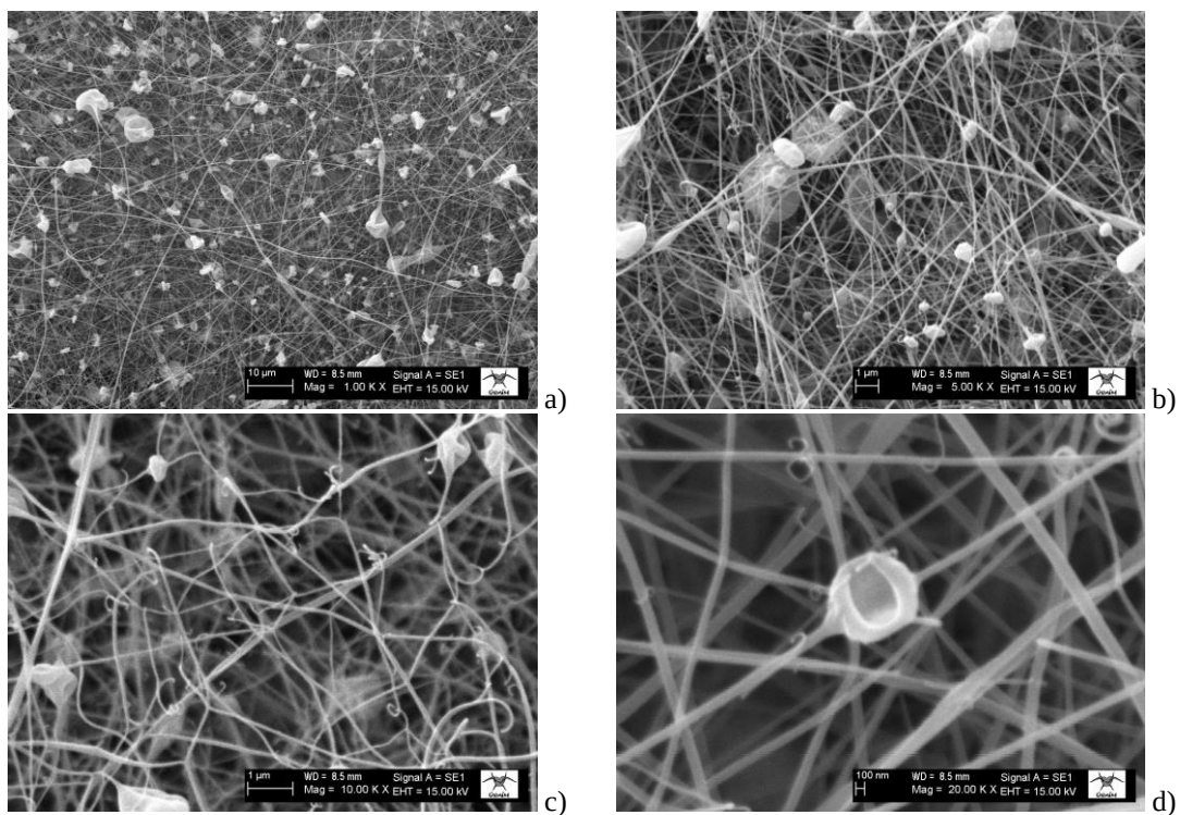
Figure 8: SEM images of P25 nanofiber surface samples at a) 1 kX, b) 5 kX, c) 10 kX and d) 20 kX
