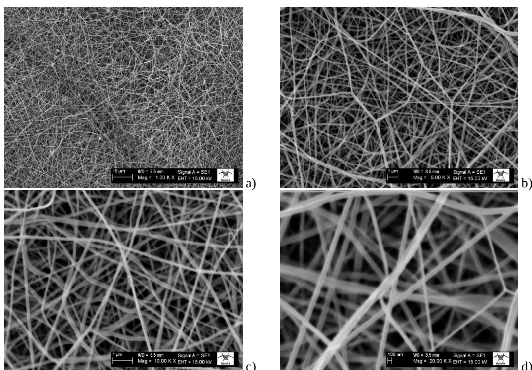
Figure 5: SEM images of P100 nanofiber surface samples at a) 1 kX, b) 5 kX, c) 10 kX and d) 20 kX
