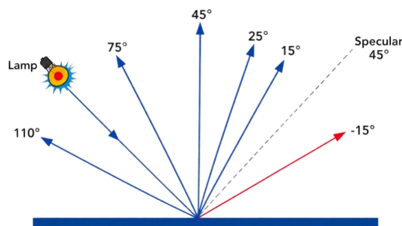
Figure 1: Example of six-angle color measurement
