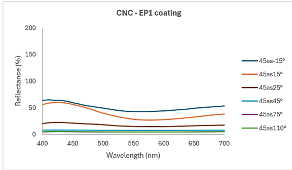
Figure 2: Reflectance spectra of CNC coating containing EP1 pigment, at different measurement geometries
