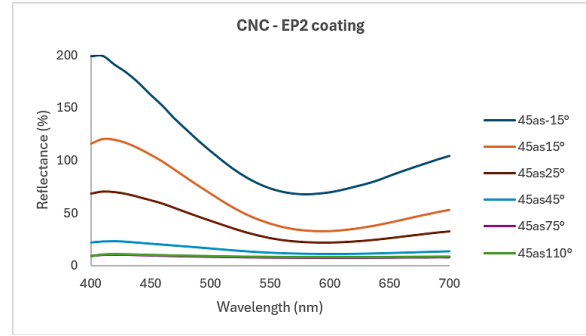
Figure 3: Reflectance spectra of CNC coating containing EP2 pigment, at different measurement geometries
