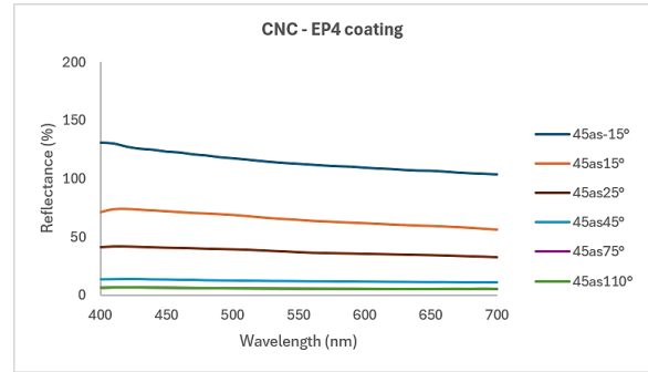
Figure 5: Reflectance spectra of CNC coating containing EP4 pigment, at different measurement geometries
