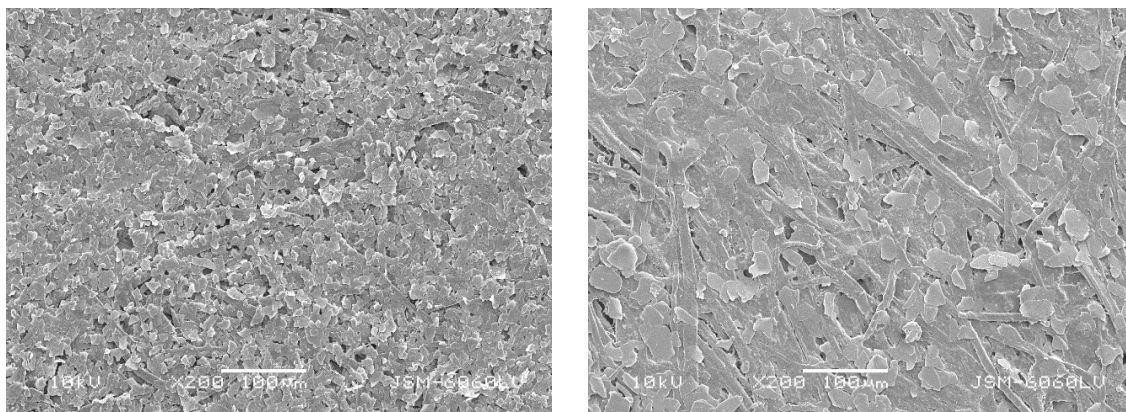
Figure 7: Scanning electron micrographs of coatings: CNC-EP3 (left) and CNC-EP4 (right)
