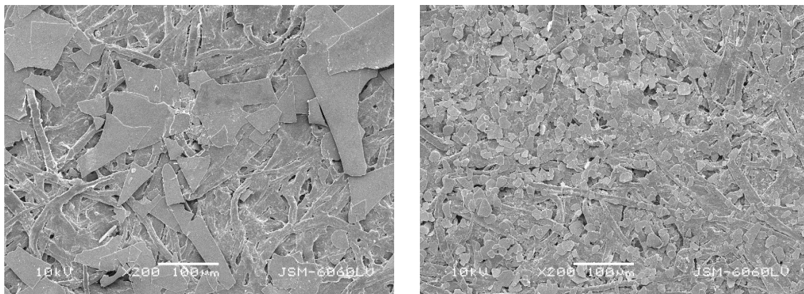
Figure 6: Scanning electron micrographs of coatings: CNC-EP1 (left) and CNC-EP2 (right)
