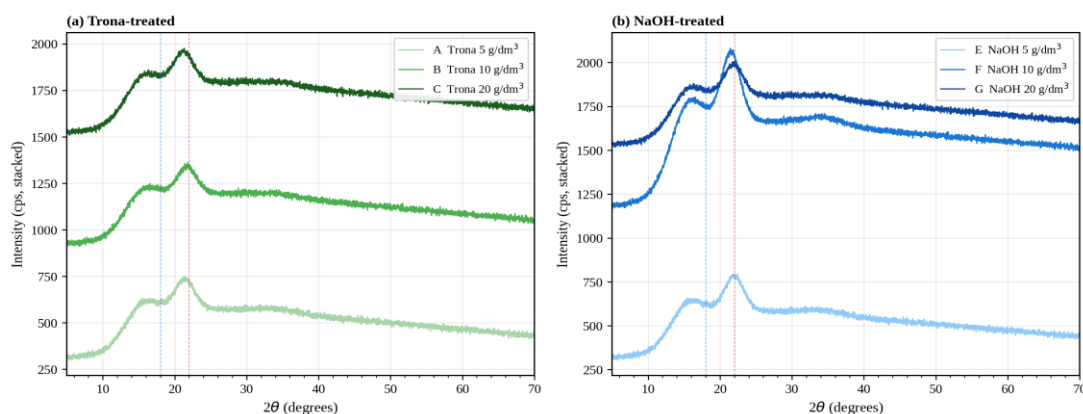
Figure 3: XRD diffractograms of the six mercerized coir samples: (a) trona-treated group (A: 5 g/dm 3 , B: 10 g/dm 3 , C: 20 g/dm 3 ), and (b) NaOH-treated group (E: 5 g/dm 3 , F: 10 g/dm 3 , G: 20 g/dm 3 ); vertical dashed lines mark the (200) crystalline peak (22°) and amorphous minimum (18°) used in the Segal calculation
