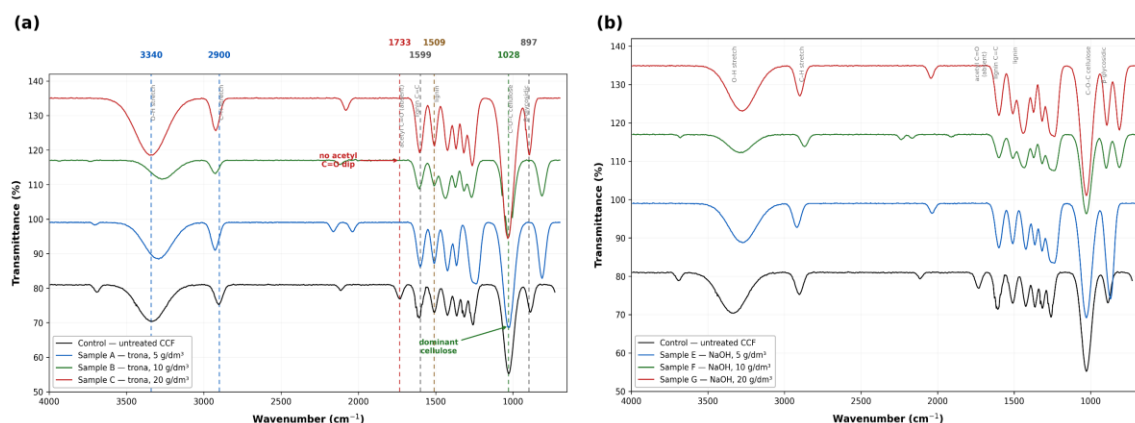
Figure 5: ATR-FTIR transmittance spectra of coir samples mercerized with (a) natural alkali trona (A: 5 g/dm 3 , B: 10 g/dm 3 , C: 20 g/dm 3 ), and (b) synthetic NaOH (E: 5 g/dm 3 , F: 10 g/dm 3 , G: 20 g/dm 3 ), each shown against the untreated raw fiber (control); vertical markers identify the acetyl C=O band of hemicelluloses (1733 cm -1 ), the aromatic C=C bands of lignin (1599 and 1509 cm -1 ) and the C–O–C glycosidic band of cellulose (1028 cm -1 )
