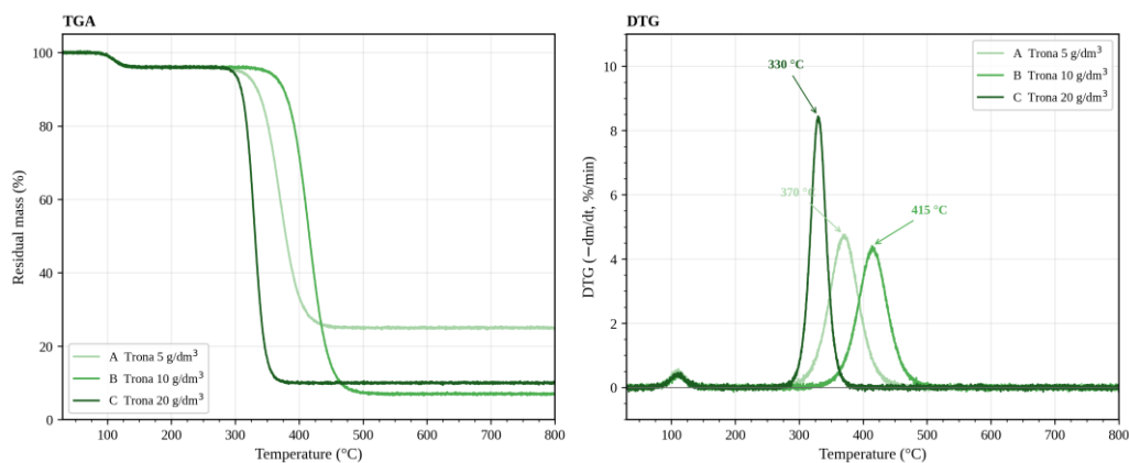
Figure 6: (Left) TGA and (right) DTG curves of trona-treated coir samples A (5 g/dm³), B (10 g/dm³) and C (20 g/dm³) recorded from 30 to 800 °C at 10 °C/min under flowing nitrogen
