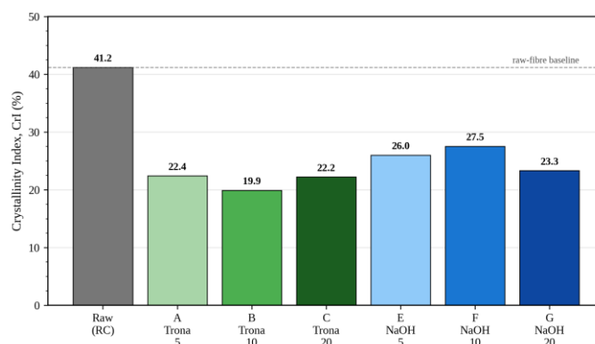
Figure 4: Comparison of the cellulose crystallinity index (CrI) of raw fiber (RC) and six mercerized coir samples (the horizontal dashed line marks the raw-fibre baseline (CrI = 41.2%))
