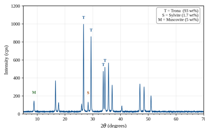
Figure 1: X-ray diffractogram of the natural alkali (Kaun bilala) recorded over 2\theta = 5\text{--}70^\circ – the pattern is dominated by sharp crystalline reflections attributable to trona (T, 93 wt%), with minor sylvite (S) and muscovite (M)
