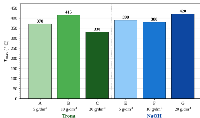
Figure 8: Comparison of the temperature of maximum mass-loss rate ( T_{\max} ) extracted from the DTG curves of the six mercerized coir samples
