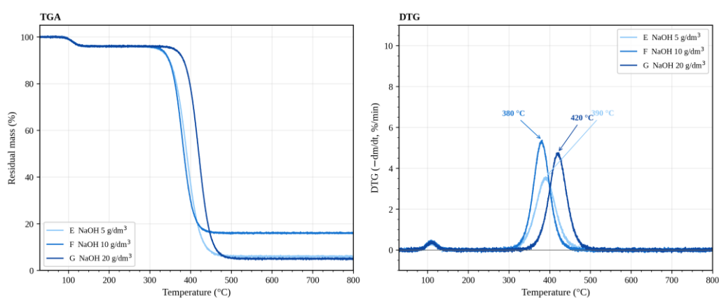
Figure 7: (Left) TGA and (right) DTG curves of NaOH-treated coir samples E (5 g/dm³), F (10 g/dm³) and G (20 g/dm³) under the same heating programme as in Figure 6
