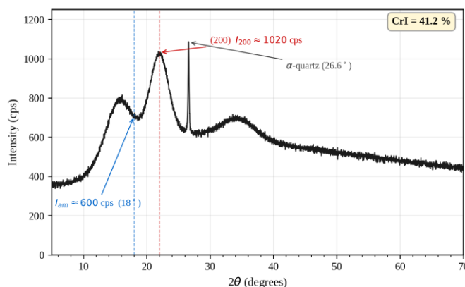
Figure 2: X-ray diffractogram of raw (untreated) coconut coir fiber over 2\theta = 5\text{--}70^\circ
