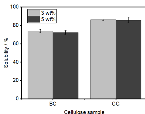
Figure 9: Comparison of cellulose solubility of BC and CC at cellulose loadings of 3 and 5 wt% (columns represent the mean values, and error bars represent the standard deviations of three independent measurements)
