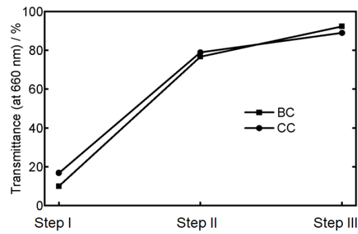
Figure 6: Transmittance including diffusely transmitted light at 660 nm of the solution at each step at feed ratio = 3%
