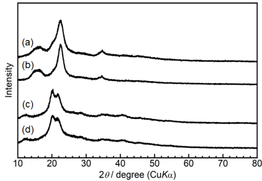
Figure 3: XRD patterns of (a) BC, (b) CC, (c) RBC and (d) RCC
