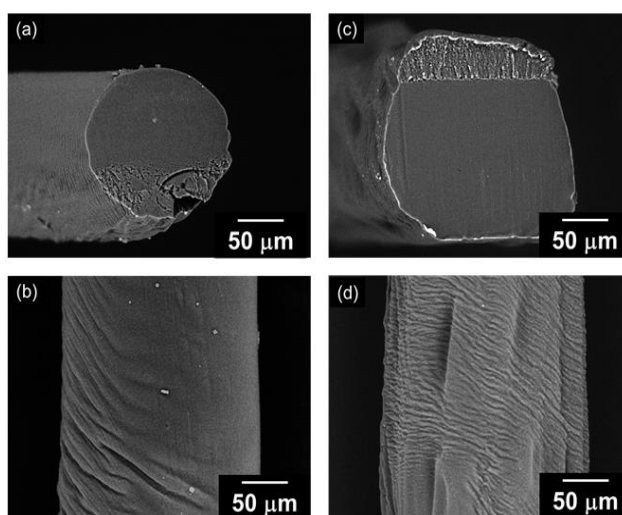
Figure 12: Representative SEM images of RBC (a, b) and RCC (c, d); cross-sectional (a, c) and side (b, d) views
