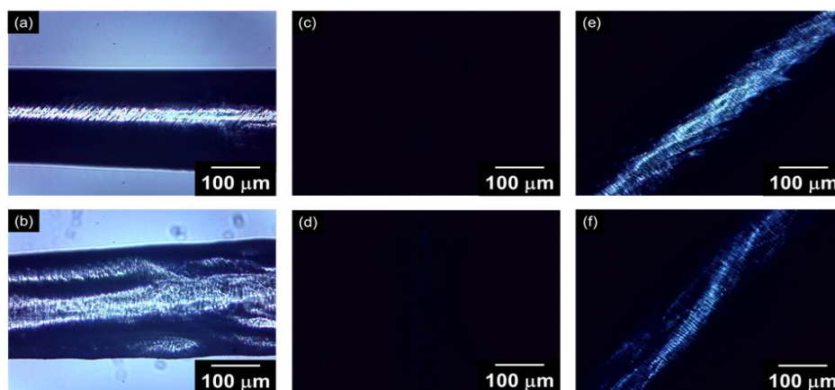
Figure 13: Optical microscopic images of RBC (a, c, e) and RCC (b, d, f) fibers; Non-polarized (a, b) and polarized observations under crossed Nicols (c, d) of fibers placed horizontally (extinction position); Polarized optical microscopic images observed under crossed Nicols (e, f) of fibers placed at 45° (diagonal position)
