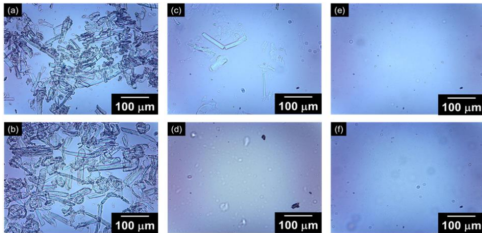
Figure 7: Optical microscopy images of the cellulose solutions at each step at feed ratio = 3%: (a) BC at step I, (b) CC at step I, (c) BC at step II, (d) CC at step II, (e) BC at step III, and (f) CC at step III
