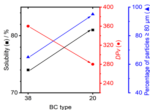
Figure 10: Solubility, DP v , and percentage of particles smaller than 80 mm for BC38 and BC20
