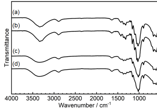
Figure 4: FT-IR spectra of (a) BC, (b) CC, (c) RBC and (d) RCC
