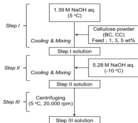
Figure 1: Flowchart for cellulose dissolution procedure
