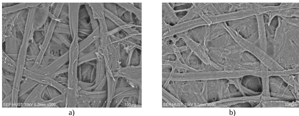
Figure 2: SEM images of paper sheets (a) without and (b) with strength additives
