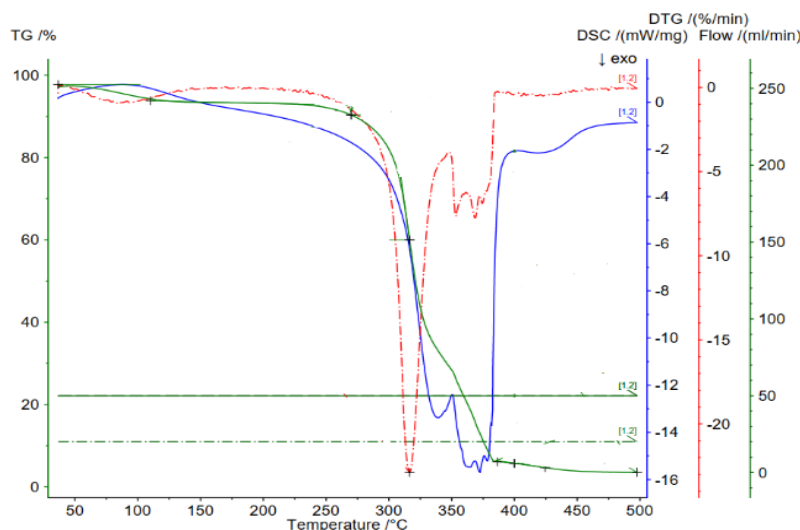
Figure 3: Thermogravimetric analysis of thermally resistant paper
