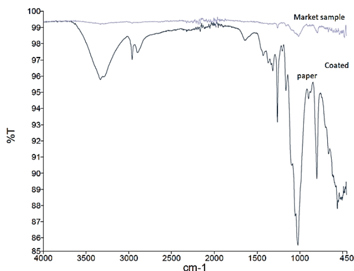
Figure 4: FTIR spectra of the market sample and coated paper
