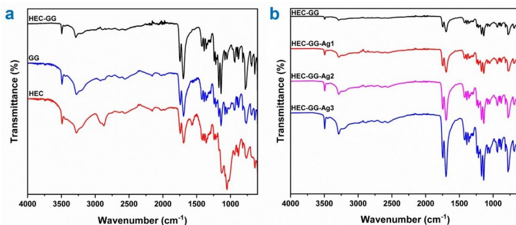
Figure 4: FTIR spectra of (a) HEC, GG, and HEC-GG sponge samples, and (b) AgNPs-loaded HEC-GG sponge samples
