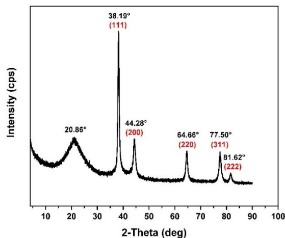
Figure 3: XRD pattern of HEC-mediated AgNPs synthesized under autoclave conditions, showing the characteristic diffraction peaks of crystalline AgNPs
