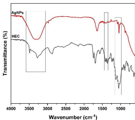
Figure 2: FTIR spectra of HEC and HEC-mediated AgNPs synthesized under autoclave conditions
