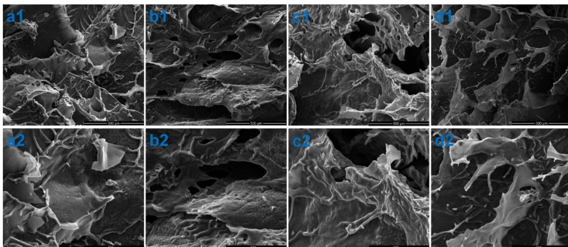
Figure 5: SEM images of sponge samples (a) HEC-GG, (b) HEC-GG-Ag1, (c) HEC-GG-Ag2, and (d) HEC-GG-Ag3 shown at two magnifications (a1-d1) 500 \mu\text{m} and (a2-d2) 200 \mu\text{m} scale bar
