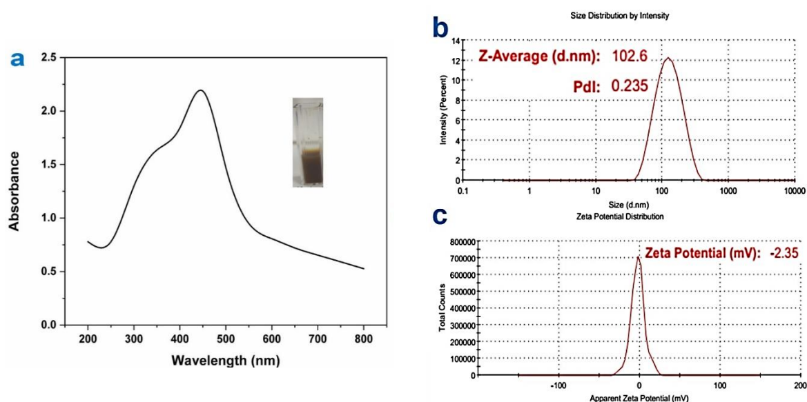
Figure 1: Characterization of HEC-mediated AgNPs synthesized under autoclave conditions: (a) UV-Vis absorption spectrum, (b) DLS particle size distribution, and (c) zeta potential analysis
