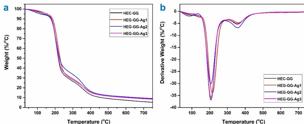
Figure 6: TGA (a) and DTG (b) curves of HEC-GG and AgNPs-loaded sponges
