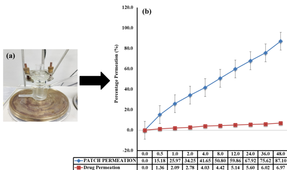
Figure 9: Ex-vivo drug permeation study, a) Franz cell and b) Permeation comparison between pure loratadine solution and prepared microneedle patch
