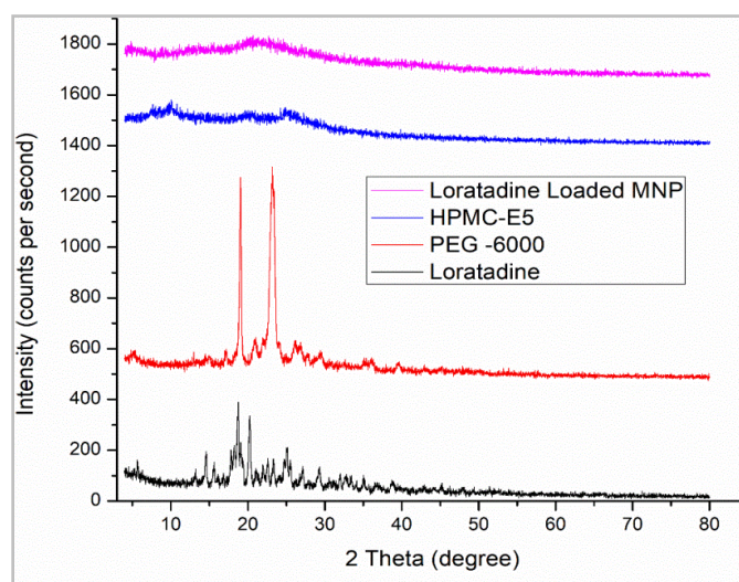
Figure 7: XRD patterns of loratadine, HPMC E5, PEG 600 and loratadine-loaded microneedle patch
