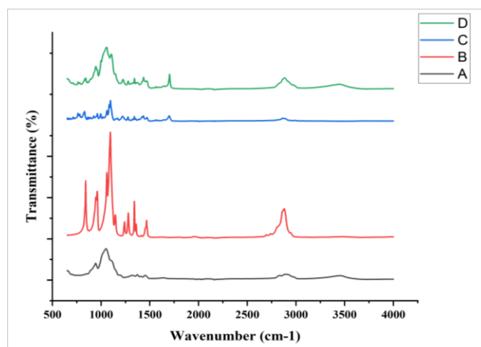
Figure 4: FTIR spectra of a) HPMC, b) PEG-6000, c) loratadine and d) loratadine-loaded microneedle patch
