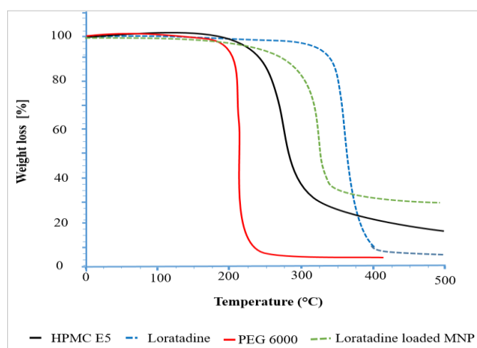
Figure 6: TGA curves of loratadine, HPMC E5, PEG 600 and loratadine-loaded microneedle patch
