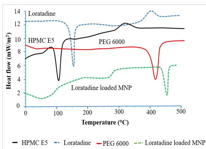
Figure 5: DSC curves of loratadine, HPMC E5, PEG 600 and loratadine-loaded microneedle patch
