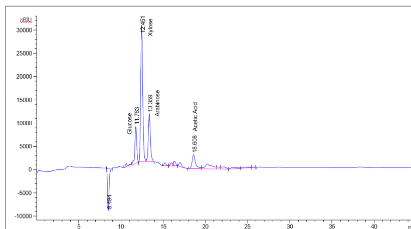
Figure 2: HPLC spectrum of pre-extracted liquor
