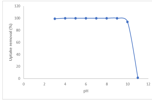
Figure 10: Effect of pH on the adsorption of RB5 by using KH-CH-ECH composite beads
