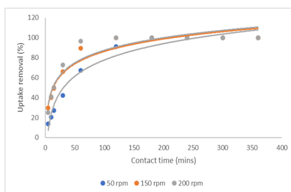
Figure 9: Effect of different agitation rates on the removal of RB5 by KH-CH-ECH composite beads
