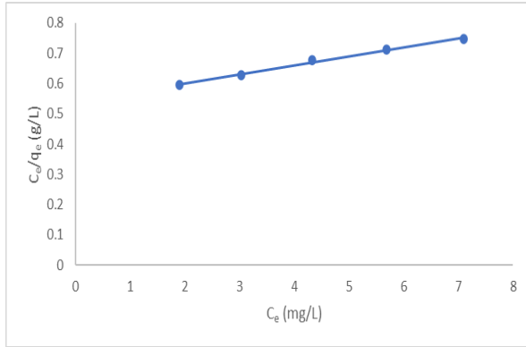
Figure 11: Langmuir isotherm plot for the removal of RB5 by KH-CH-ECH composite beads
