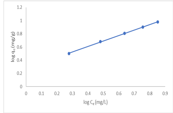
Figure 12: Freundlich isotherm plot for the removal of RB5 by KH-CH-ECH composite beads
