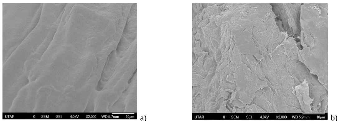
Figure 3: SEM micrographs of KH-CH-ECH composite beads (a) before and (b) after the adsorption of RB5
