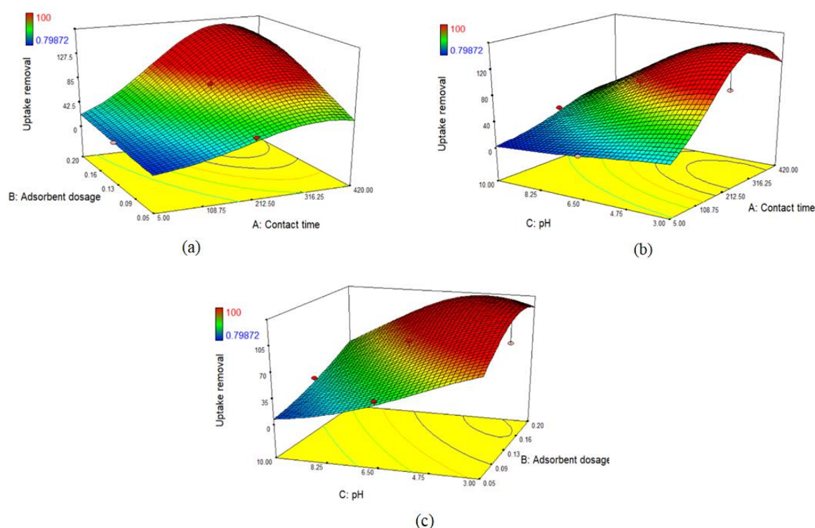
Figure 15: Response surface plots of the interaction effects between (a) contact time and adsorbent dosage, (b) contact time and pH, and (c) adsorbent dosage and pH on uptake removal of RB5
