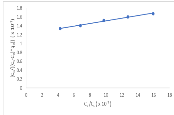
Figure 13: BET isotherm plot for the removal of RB5 by KH-CH-ECH composite beads
