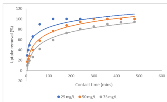
Figure 6: Effect of contact time and initial RB5 concentration on adsorption performance
