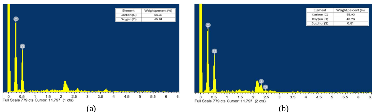
Figure 4: EDX spectra of KH-CH-ECH composite beads (a) before and (b) after the adsorption of RB5
