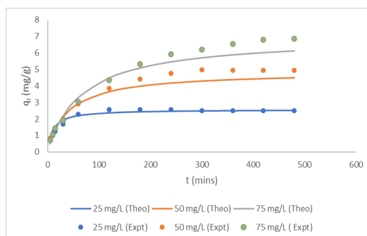
Figure 14: Comparison between theoretical and experimental adsorption capacity (pseudo-second order)
