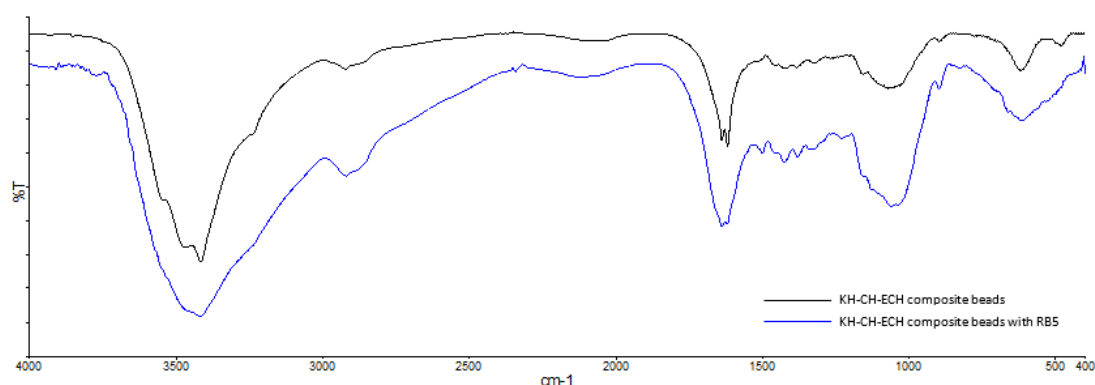
Figure 2: ATR-FTIR spectra of KH-CH-ECH composite beads before and after the adsorption of RB5
