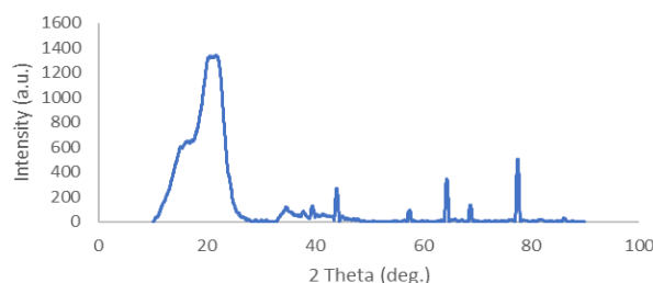
Figure 1: XRD pattern of KH-CH-ECH composite beads
