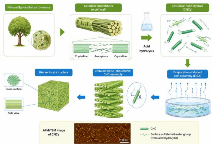
Figure 3: Flowchart of the CNC fabrication process
