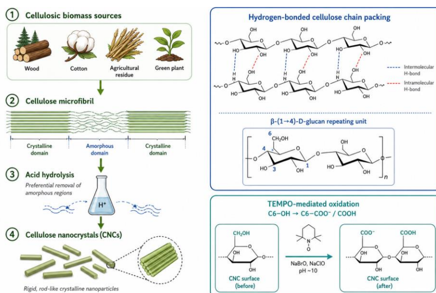
Figure 5: Preparation of CNCs via TEMPO oxidation and their chemical structures
