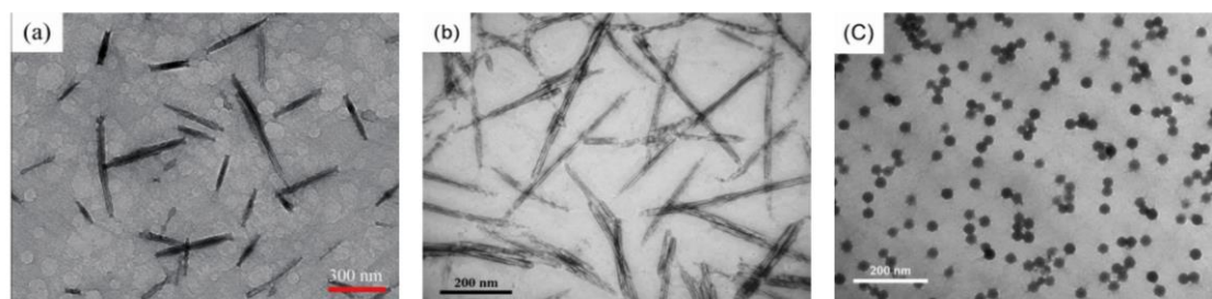
Figure 2: Rod-like (a), needle-like (b), and spherical (c) morphologies of CNCs (SEM images in panels (a–c) are original, acquired by the author, not reproduced from published literature)
