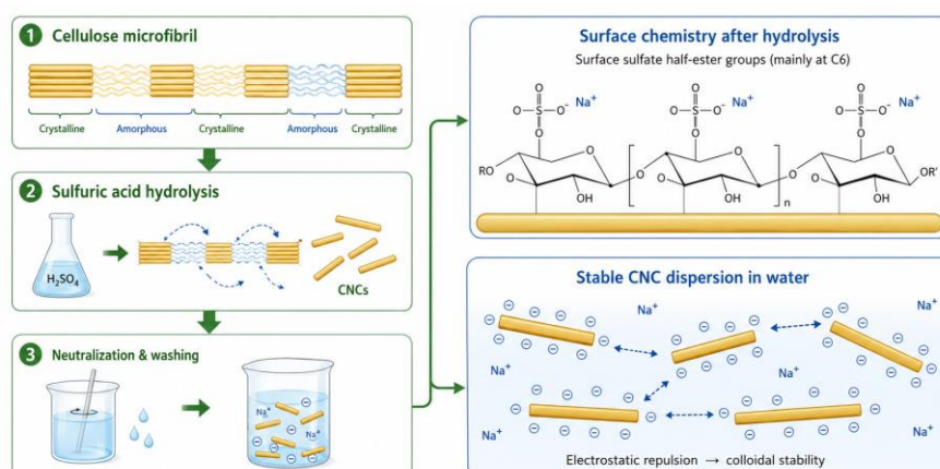
Figure 4: Isolation of CNCs from cellulose via sulfate hydrolysis
