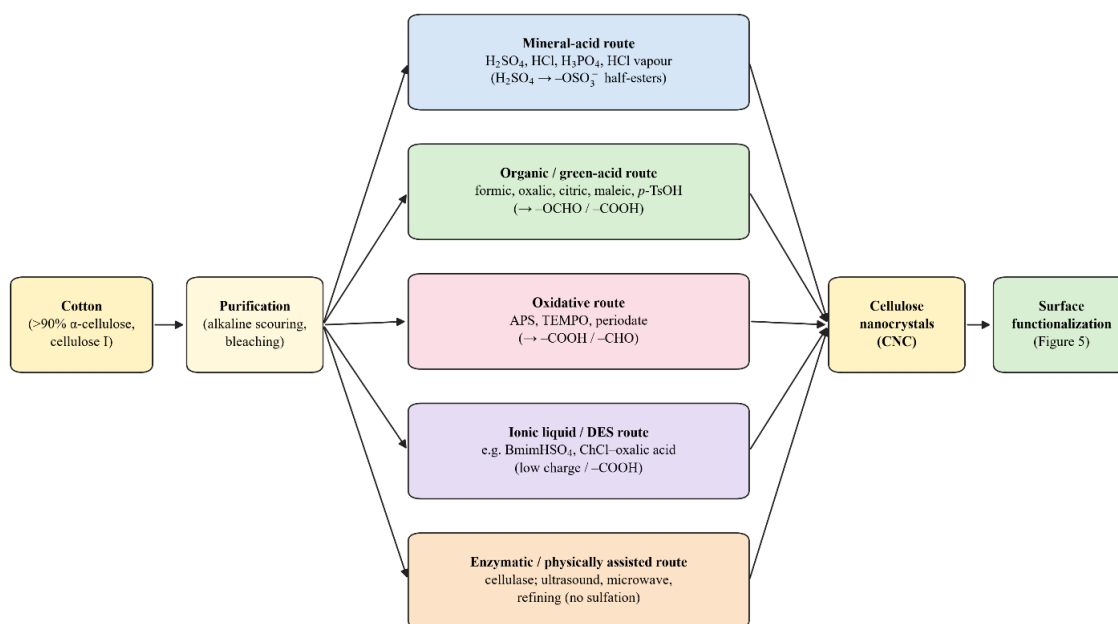
Figure 3: Extraction routes of cellulose nanocrystals from cotton: mineral-acid, organic/green-acid, oxidative, ionic-liquid/DES and enzymatic/physically assisted (ultrasound, microwave, refining) pathways, leading to CNCs and onward surface functionalization
