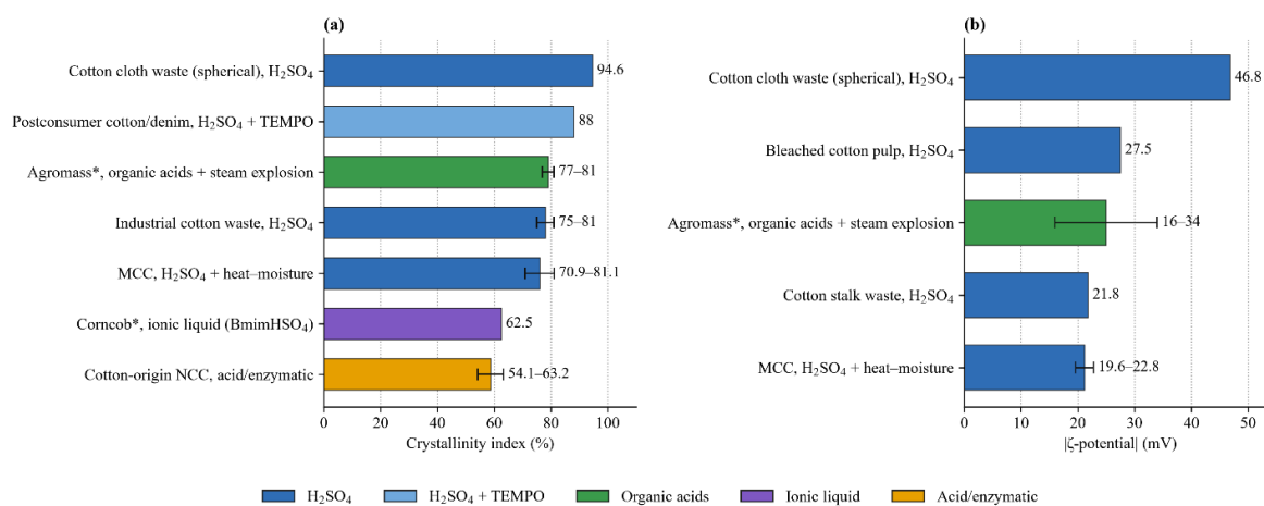
Figure 4: Literature-reported crystallinity index (a) and magnitude of the ζ-potential (b) of CNCs from cotton and closely related feedstocks, grouped by isolation route (data from Table 4). Bars show single reported values or range midpoints, and whiskers indicate the reported ranges; * denotes a closely related (non-cotton) feedstock. The gaseous-HCl route gives essentially uncharged CNCs for which no ζ-potential value was reported, and it is therefore not shown in (b)
