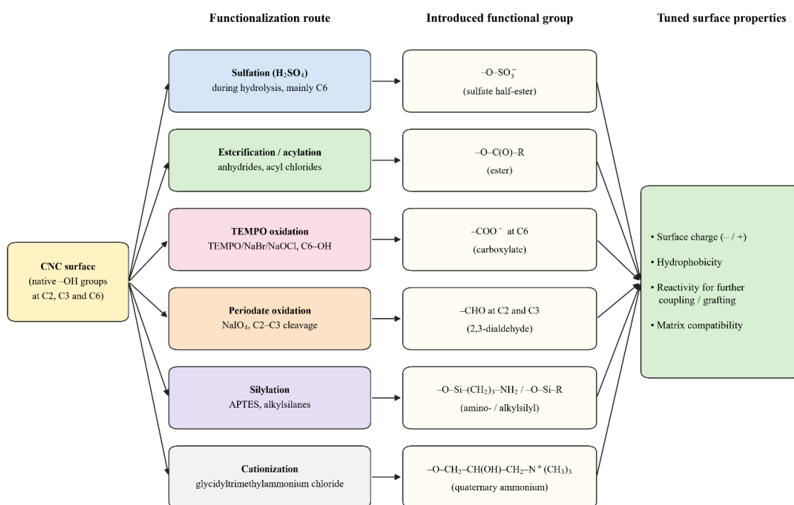
Figure 5: Surface functionalization of cotton-derived CNCs: the native hydroxyl surface is converted by sulfation, esterification, TEMPO/periodate oxidation, silylation or cationization into defined functional groups that tune charge, hydrophobicity, reactivity and matrix compatibility
