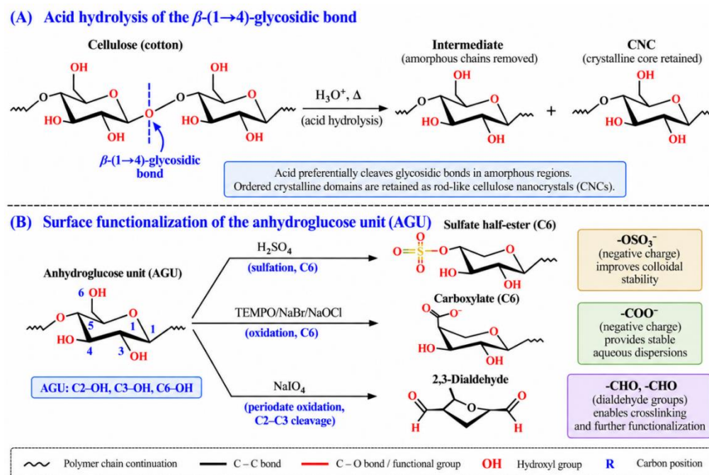
Figure 2: Key reaction chemistry of CNC from cotton: (A) acid hydrolysis of \beta -(1 \rightarrow 4)-glycosidic bonds, which removes accessible amorphous chains and leaves the crystalline core; (B) surface functionalization of the anhydroglucose unit – sulfation (C6 \rightarrow -\text{OSO}_3^- ), TEMPO oxidation (C6 \rightarrow -\text{COO}^- ) and periodate oxidation (C2–C3 cleavage \rightarrow 2,3-dialdehyde)
