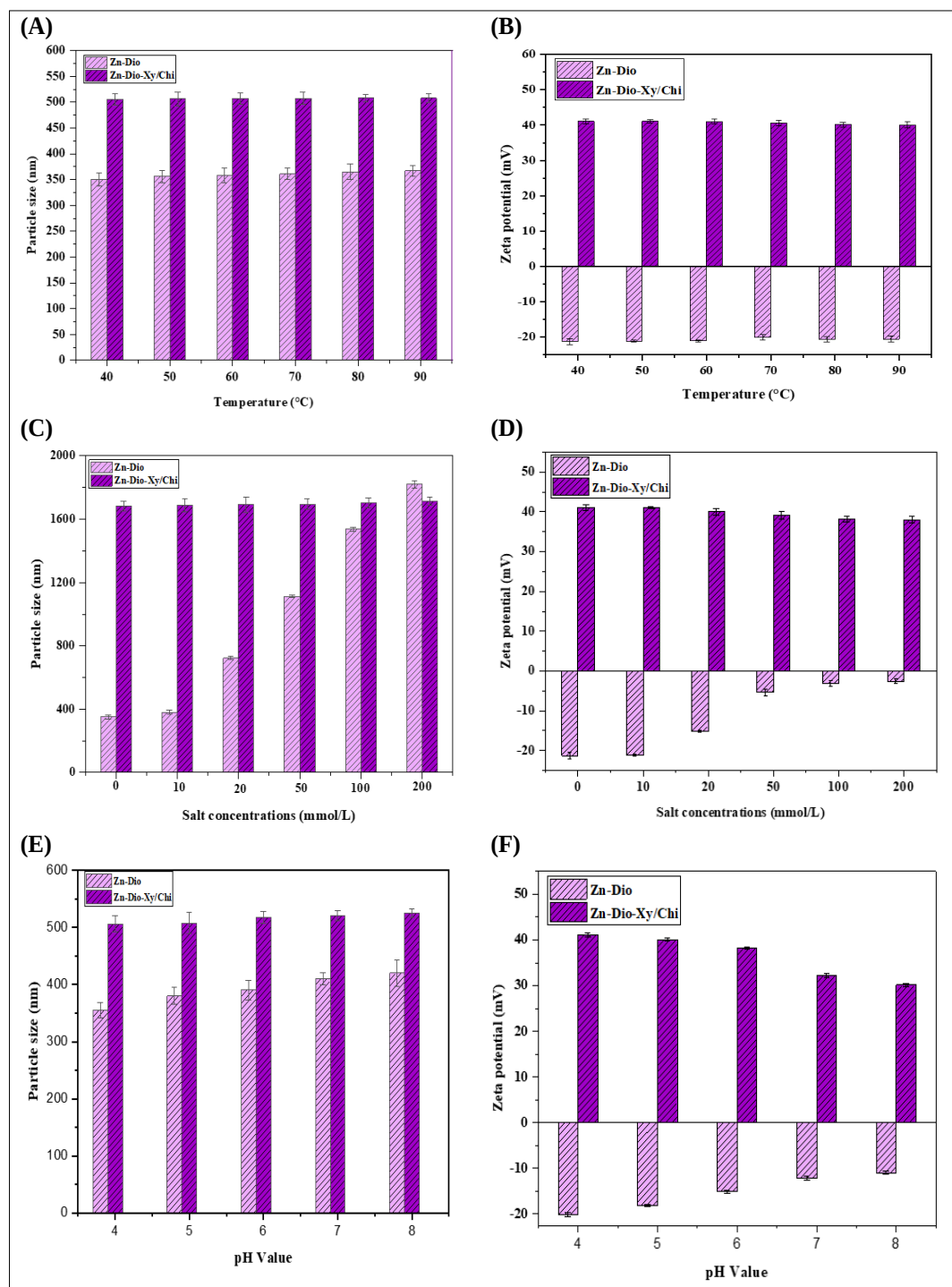
Figure 7: Thermal stability of Zn-Dio and Zn-Dio-Xy/Chi: (A) Particle size, and (B) Zeta-potential; Ionic stability of Zn-Dio and Zn-Dio-Xy/Chi: (C) Particle size, (D) Zeta-potential; pH stability of Zn-Dio and Zn-Dio-Xy/Chi: (E) Particle size and (F) Zeta-potential
