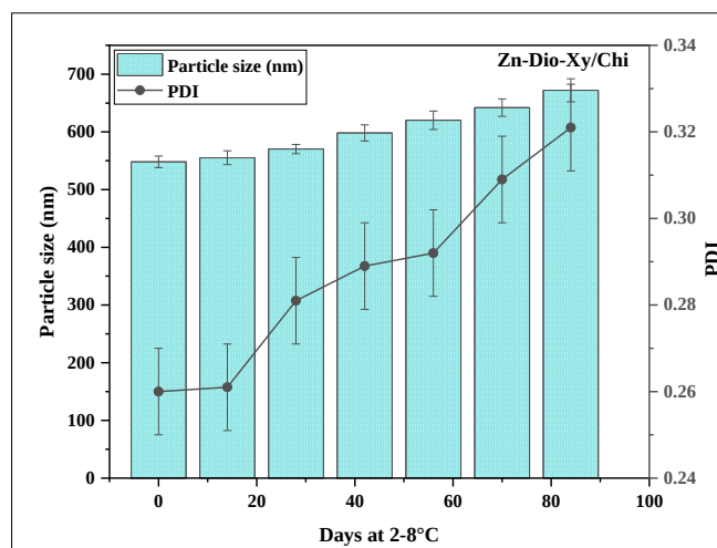
Figure 8: Storage stability of Zn-Dio-Xy/Chi
