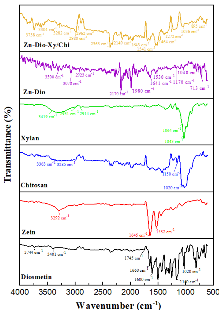
Figure 6: FTIR spectra of Dio, Xy, Zn, Zn-Dio, Chi and Zn-Dio-Xy/Chi nanoparticles
