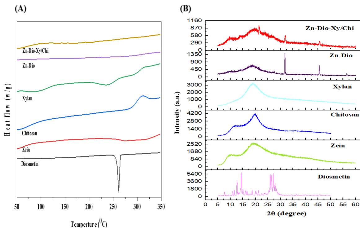
Figure 5: Thermograms (A) and diffractograms (B) of Dio, Xy, Zn, Zn-Dio, Chi and Zn-Dio-Xy/Chi nanoparticles
