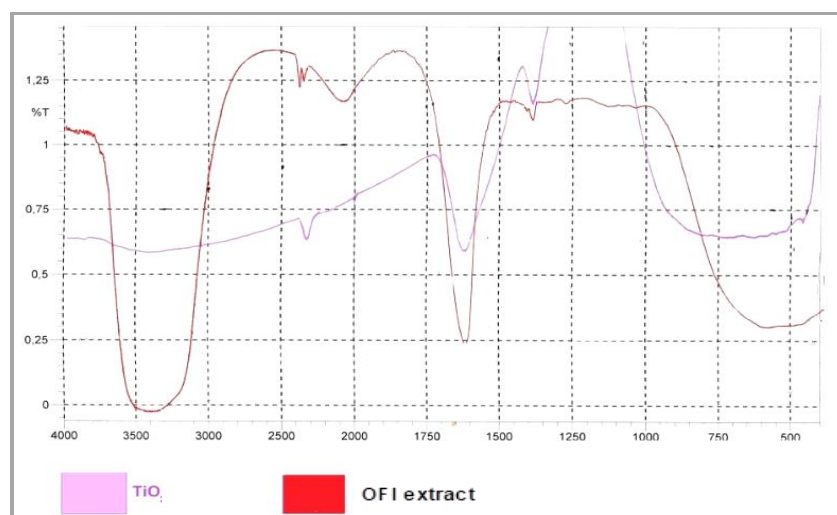
Figure 4: FT-IR spectra of the peel extract of Opuntia ficus indica and of TiO 2 NPs synthesized using the extract
