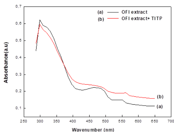
Figure 5: UV-Vis spectra of the peel extract of Opuntia ficus indica and of TiO 2 NPs synthesized using the extract
