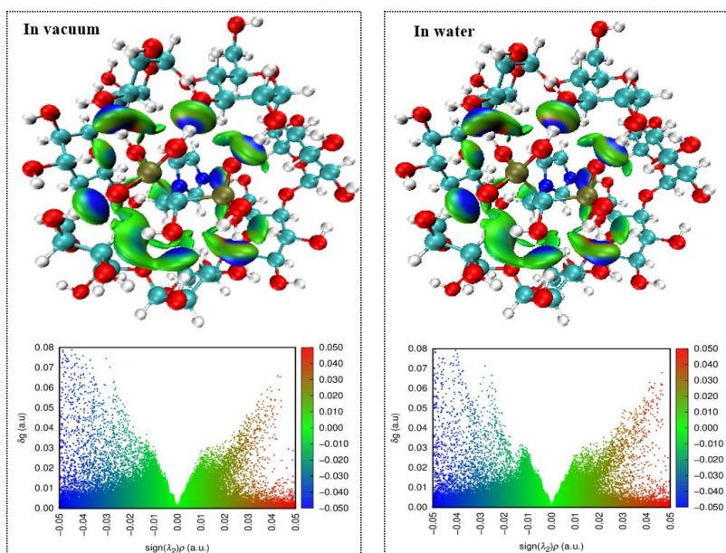
Figure 6: IGM isosurfaces and scatter plots of ZA@ \beta -CD (Configuration A)
