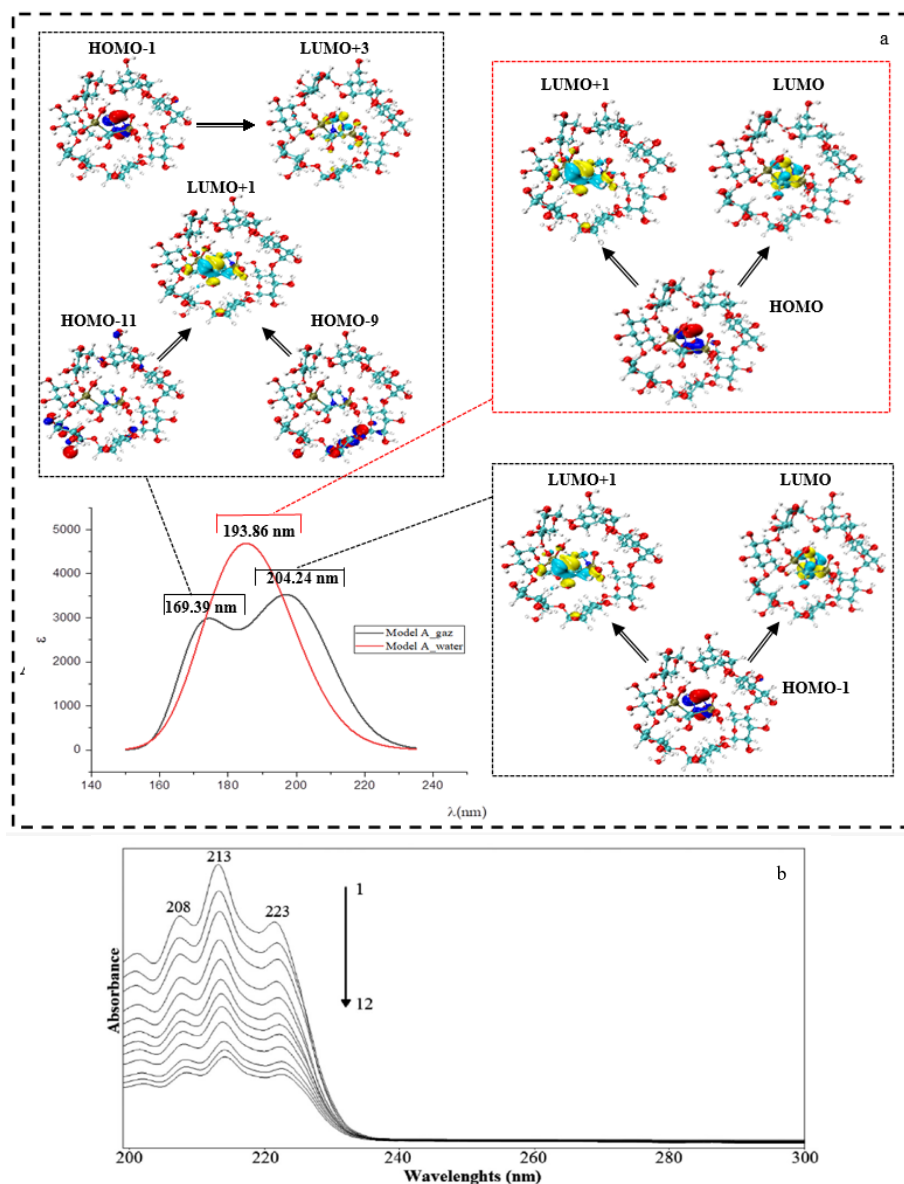
Figure 7: UV-Vis absorption spectra of the ZA@ \beta -CD inclusion complex: (a) Theoretical TD-DFT spectrum computed in the aqueous phase; (b) Experimental spectrum, reproduced from Dikmen 9
