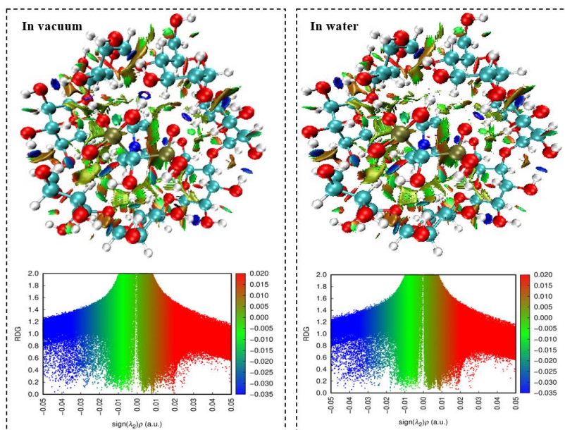
Figure 5: Scatter plots together with the color-filled NCI-RDG isosurfaces of ZA@ \beta -CD (Configuration A)
