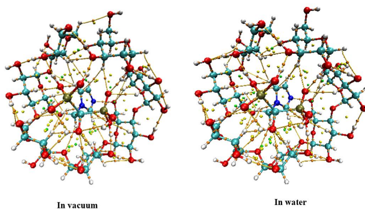
Figure 4: Molecular topology analysis of ZA@β-CD (Configuration A)
