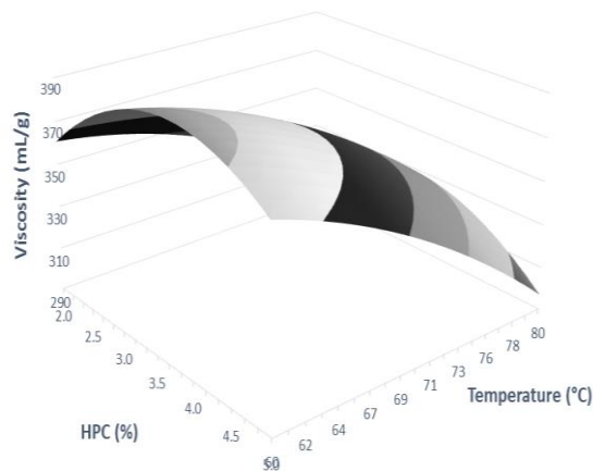
Figure 3: Viscosity variations at different temperature and hydrogen peroxide content (HPC)
