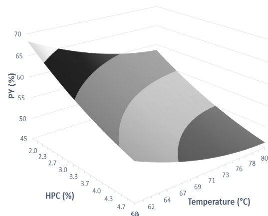
Figure 4: Pulp yield variations at different temperature and hydrogen peroxide content (HPC)
