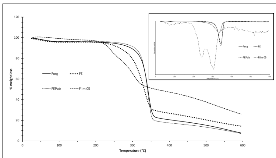
Figure 10: Thermogravimetry analysis of organosolv pulp (Forg), pulp after alkaline process (FE), bleached pulp (FEPab) and nanocellulose obtained after 5 homogenizer passes (Film 05)
