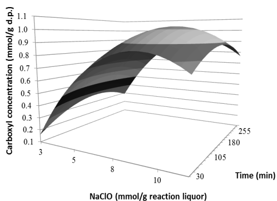
Figure 5: Effect of NaClO content and reaction time on carboxyl formation
