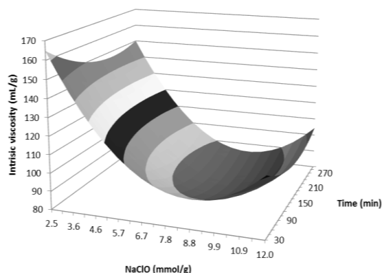
Figure 6: Effect of NaClO and time variations on intrinsic viscosity
