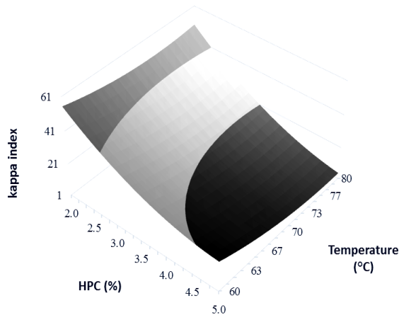
Figure 1: Effect of hydrogen peroxide and temperature variations on kappa index
