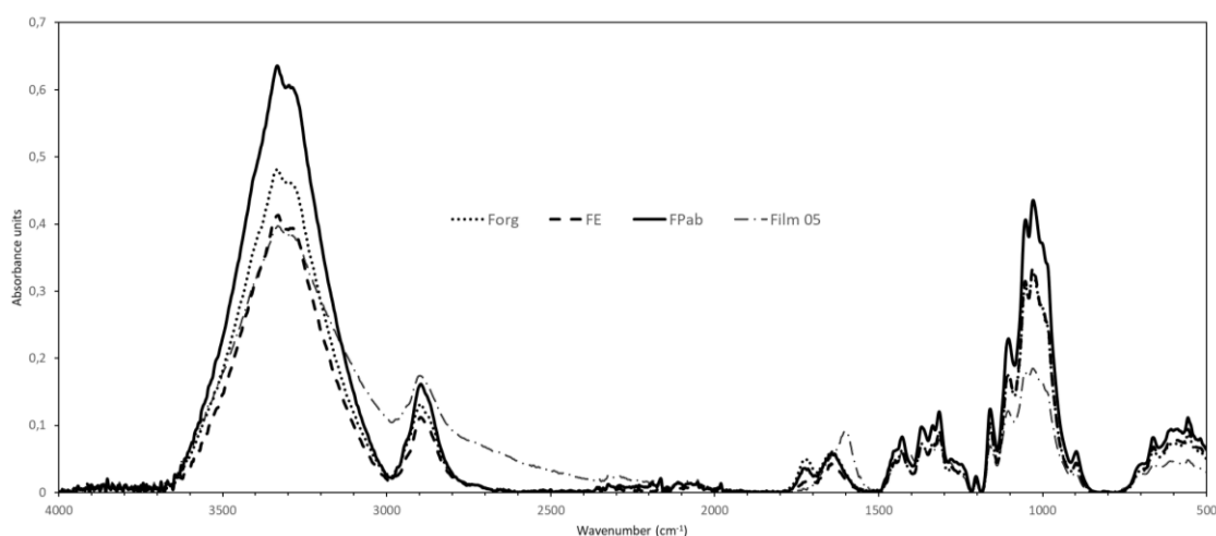
Figure 9: FTIR-ATR spectra of organosolv pulp (Forg), pulp after alkaline process (FE), bleached pulp (FEPab) and nanocellulose obtained after 5 homogenizer passes (Film 05)
