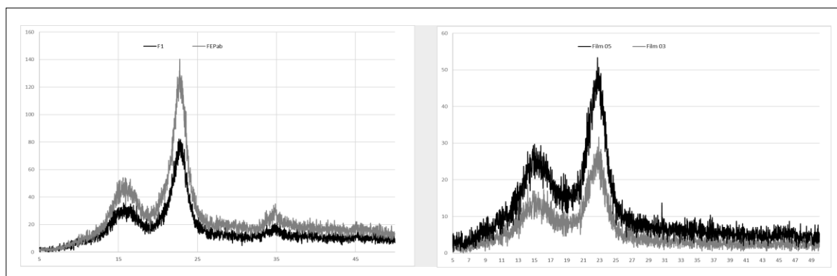
Figure 11: X-ray diffraction patterns of organosolv pulp (F1), bleached pulp (FEPab), and nanocellulose obtained after 3 and 5 homogenizer passes (Films 03 and 05)
