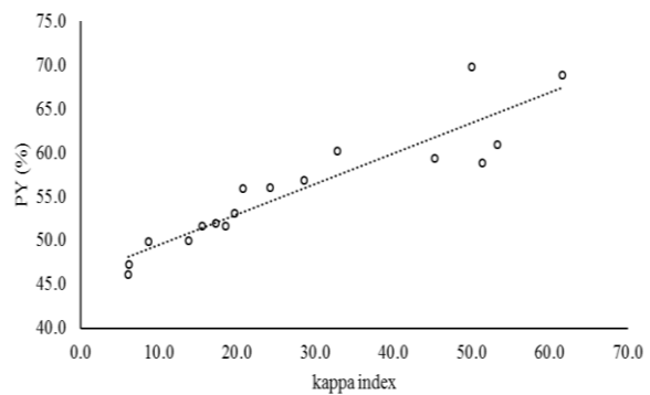
Figure 2: Kappa index versus pulp yield in performic acid treatment
