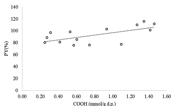
Figure 7: Relationship between PY and concentration of carboxyl groups
