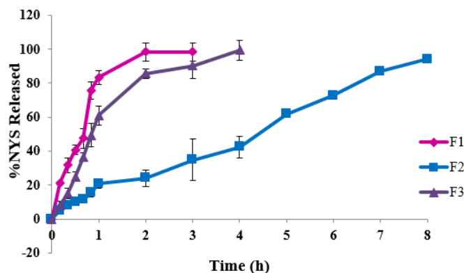
Figure 6: % NYS release of the prepared films, where F1 – NYS loaded in CMC, F2 – NYS loaded in CMC:HEC, and F3 – NYS loaded in HEC; data presented as mean ± SD, (n = 3)
