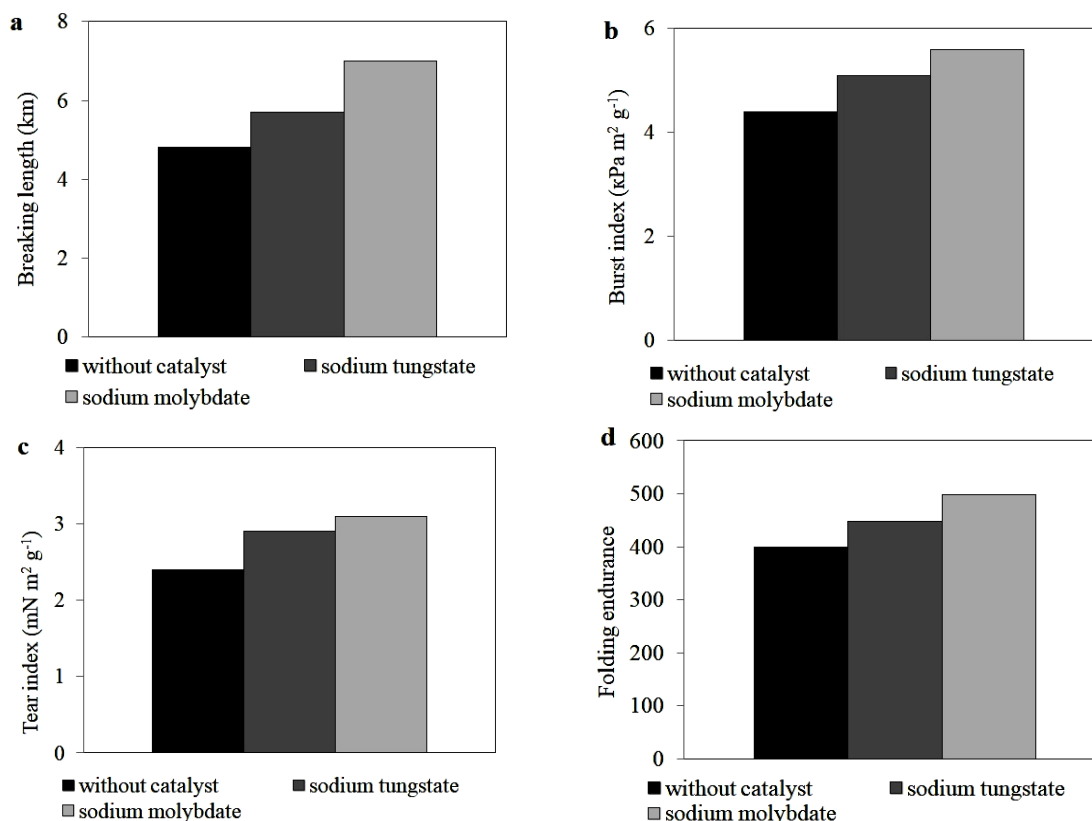
Figure 2: Physical properties of peracetic pulps: breaking length (a), burst index (b) and tear index (c)
