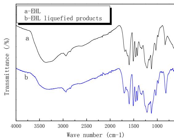
Figure 1: FTIR spectra of (a) EHL and (b) EHL liquefied products
