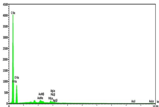
Figure 5: EDX spectrograms of CNW/palladium phenanthroline complex
