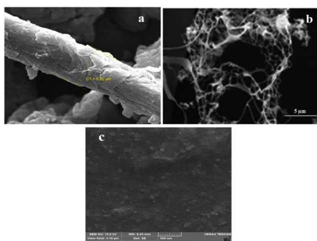
Figure 4: SEM images of cotton linter (a), cellulose nanowhisker (b) and palladium complex/cellulose nanocrystal (c)
