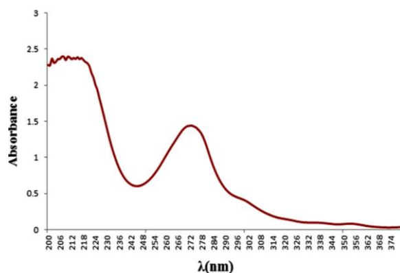
Figure 2: UV-visible absorption spectrum of palladium phenanthroline complex
