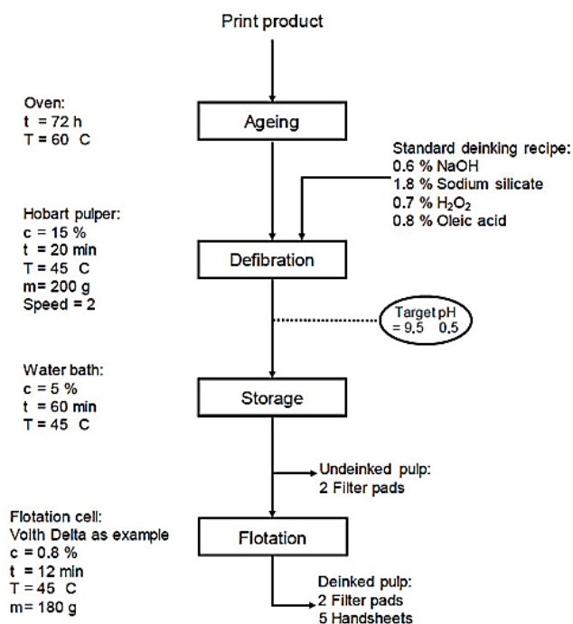
Figure 1: Flow chart of INGEDE method 11p 12
