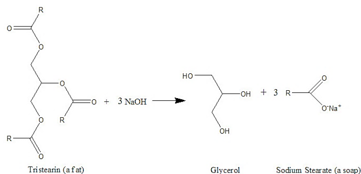
Figure 3: General saponification reaction of triglycerides resulting in sodium soap and glycerin
