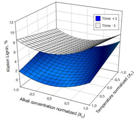
Figure 3: Variation of Klason lignin as a function of alkali concentration ( X_C ) and pulping temperature ( X_T ) at two time operation levels
